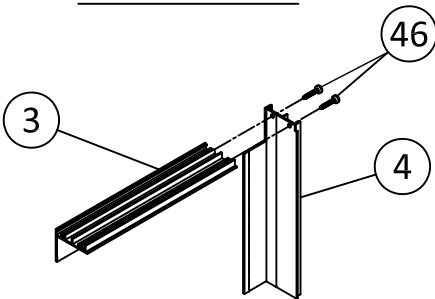
FLAT FRAME CORNER CONSTRUCTION
