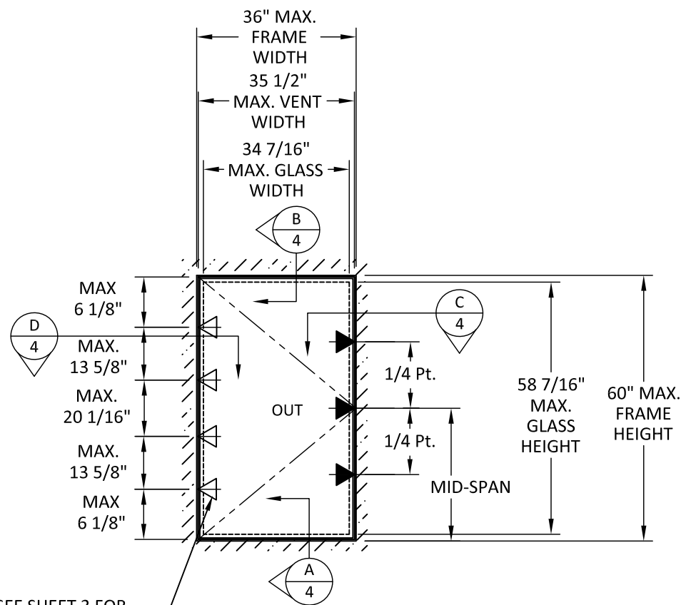
ELEVATION MULTI-POINT LOCK
