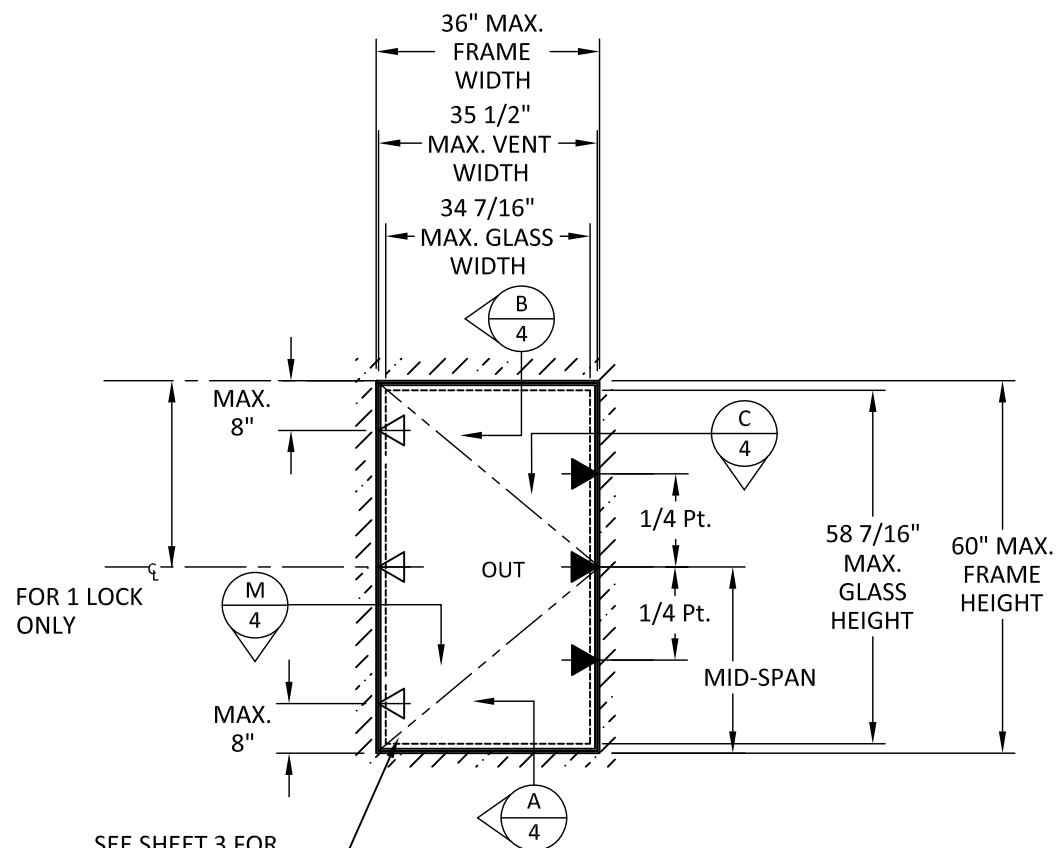
ELEVATION CAM LOCK
