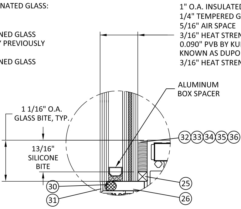
GLAZING DETAIL 3
