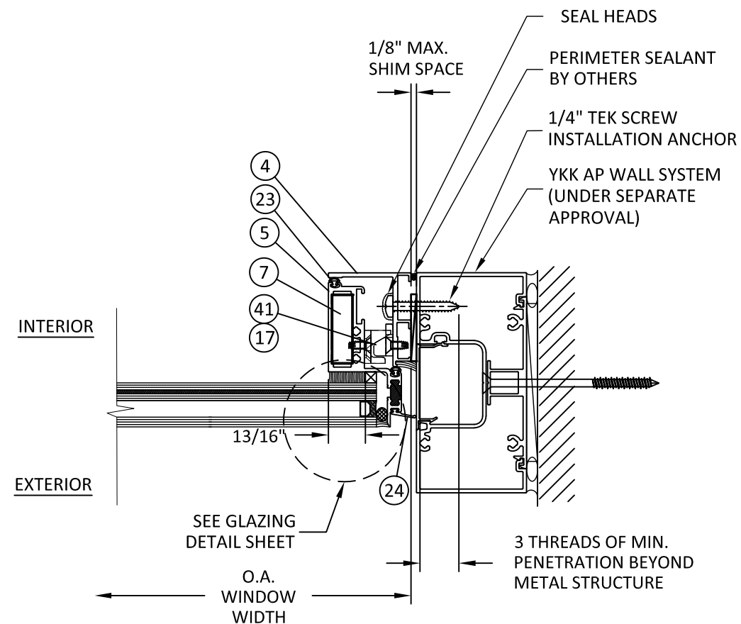
G 5 HORIZONTAL SECTION VENT JAMB - YKK AP WALL SYSTEM FLAT FRAME
