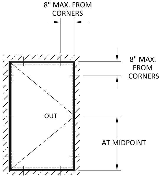
ANCHOR LAYOUT POCKET FRAME
