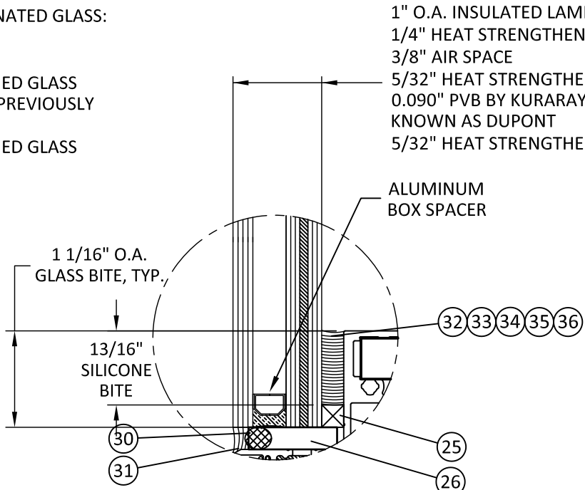
GLAZING DETAIL 4
