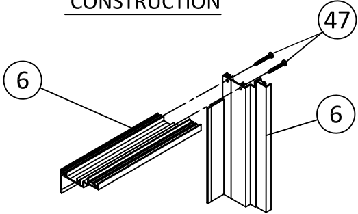
POCKET FRAME CORNER CONSTRUCTION
