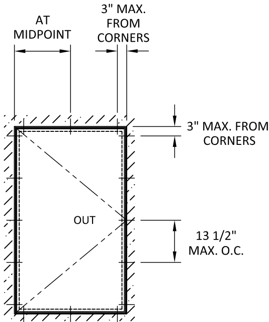
ANCHOR LAYOUT FLAT FRAME
