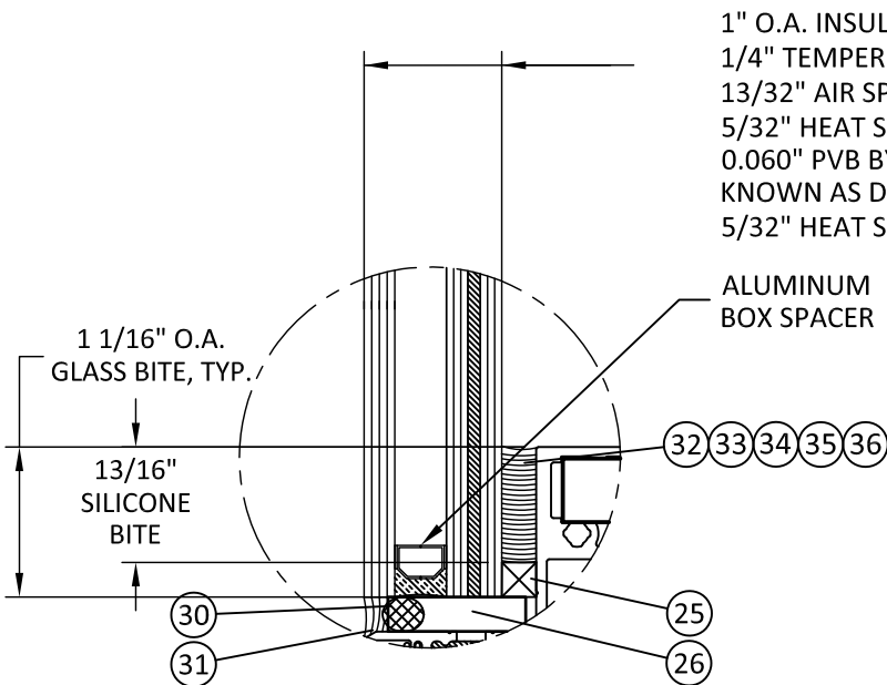
GLAZING DETAIL 2
