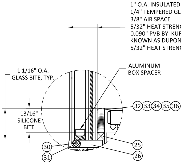
GLAZING DETAIL 1
